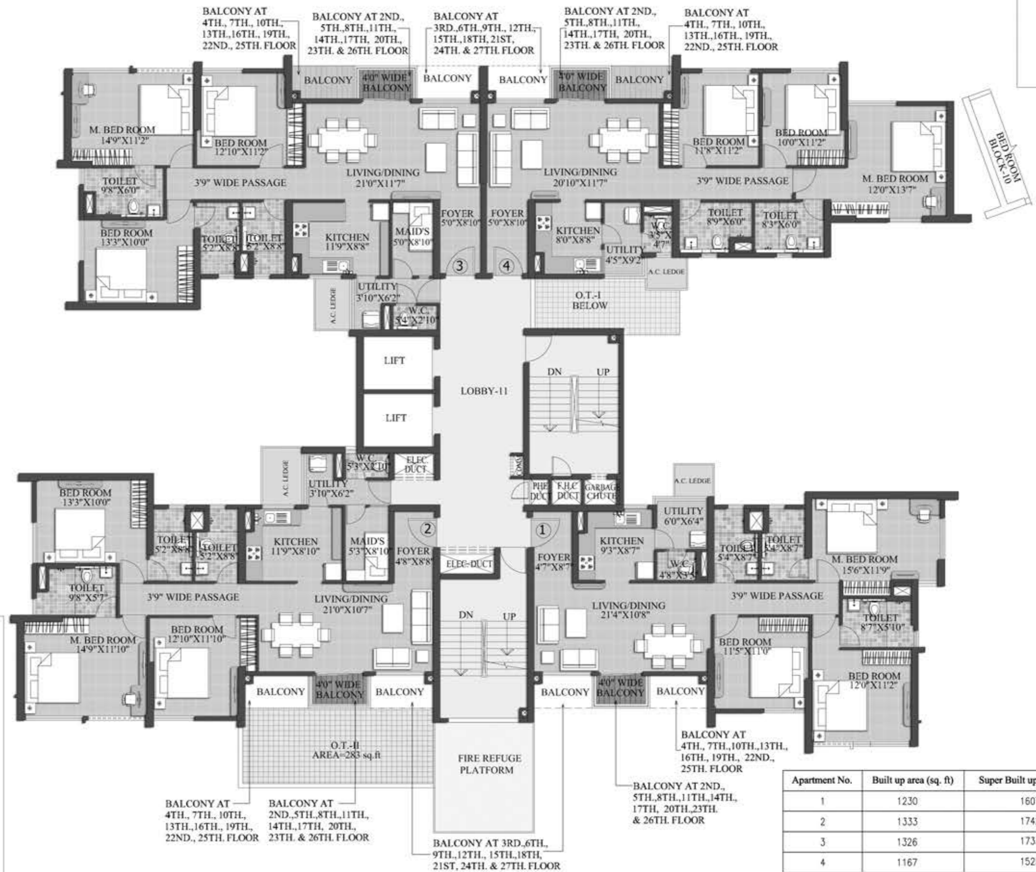
LAYOUT PLAN
